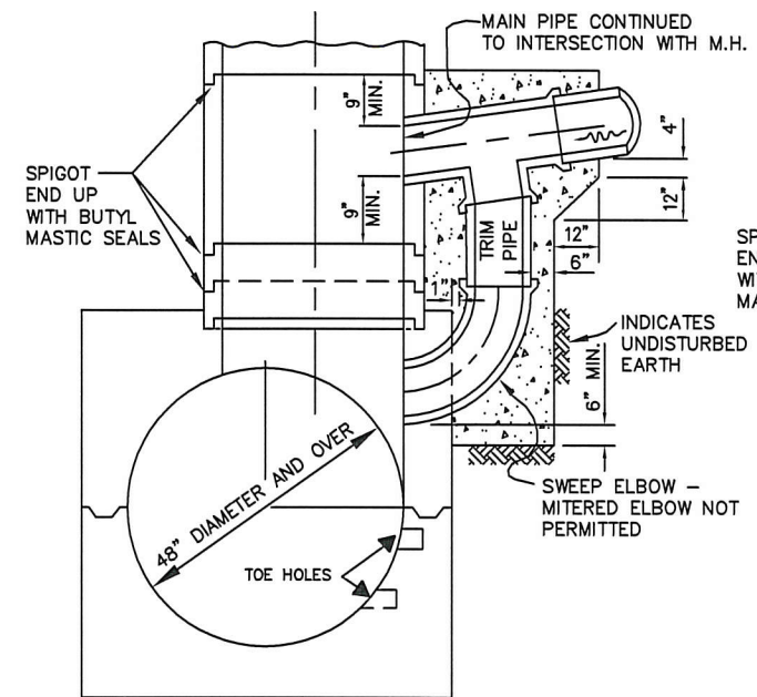
SECTION A-A TYPE "D" OR "T"
